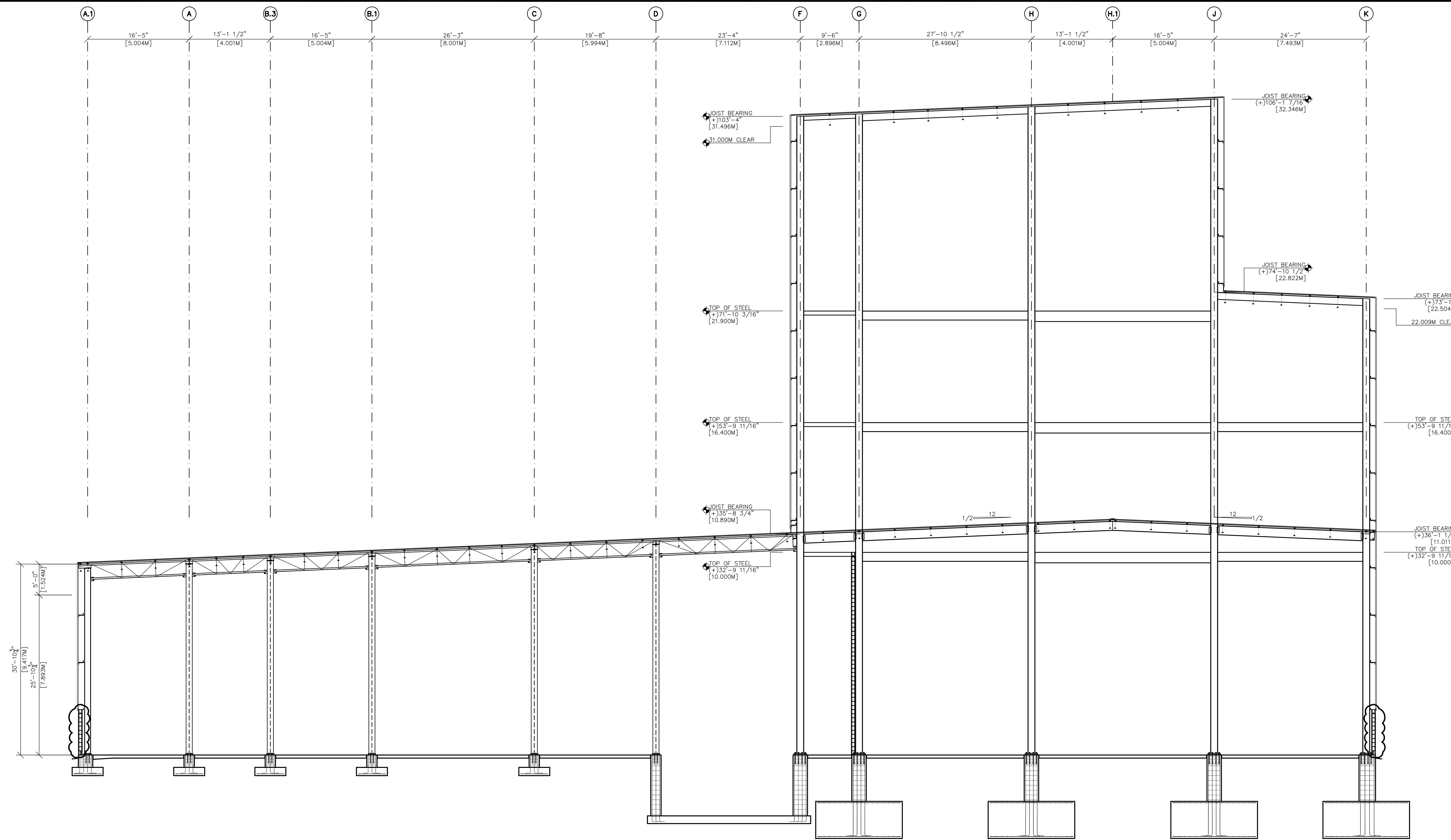
1 SECTION S-301 GRIDLINES 5 - 5
